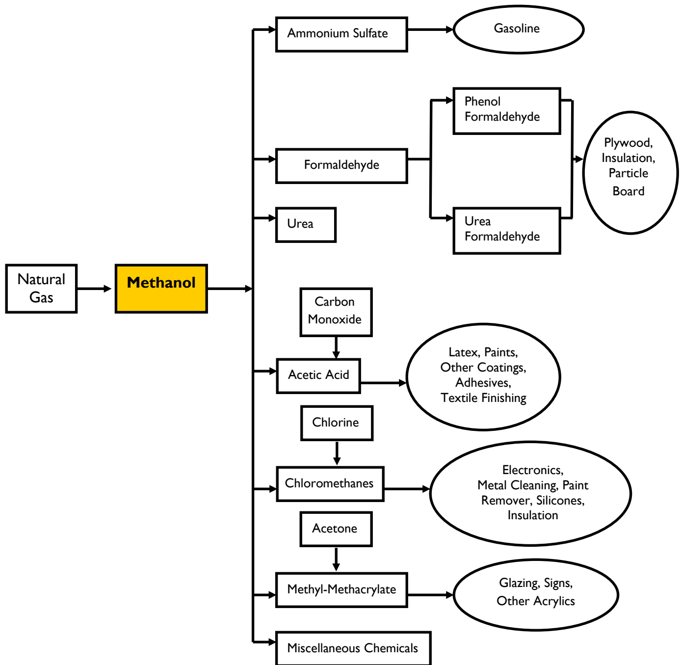
FIGURE 2.5 Methanol Chain
