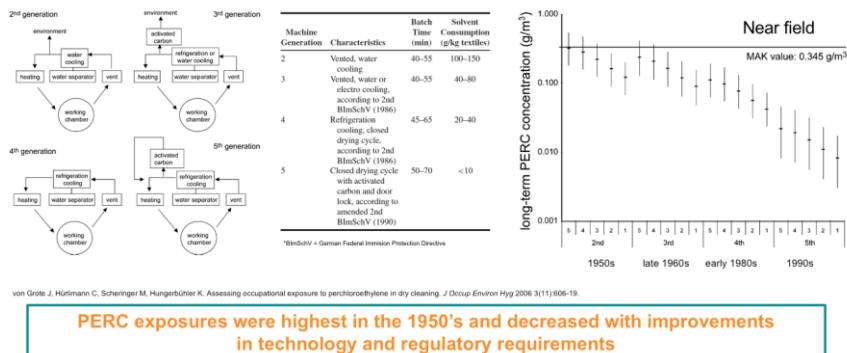
Figure 3. Historical occupational exposure trends, Example 2: PERC levels by dry cleaner type and size. Source: von Grote et al. (2006).
